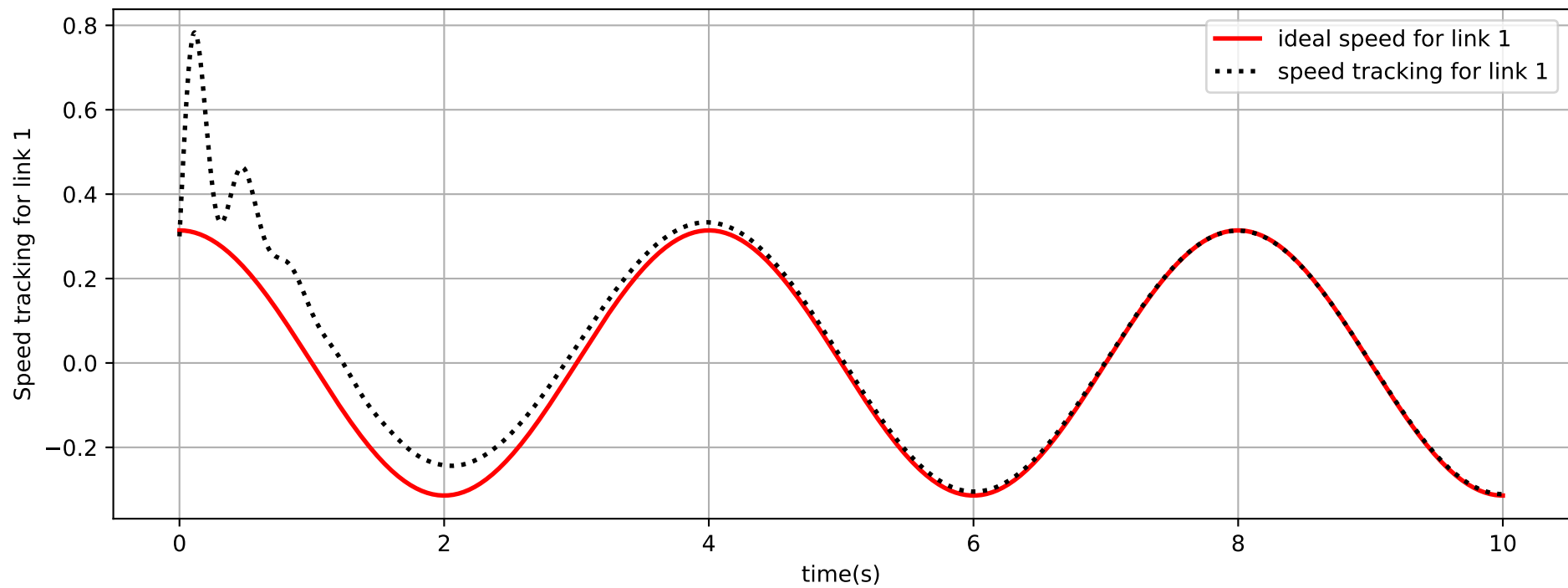
Speed Tracking Performance ( S=3 , S1=1 , m=5 )
